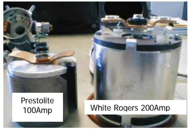
Prestolite 100Amp
